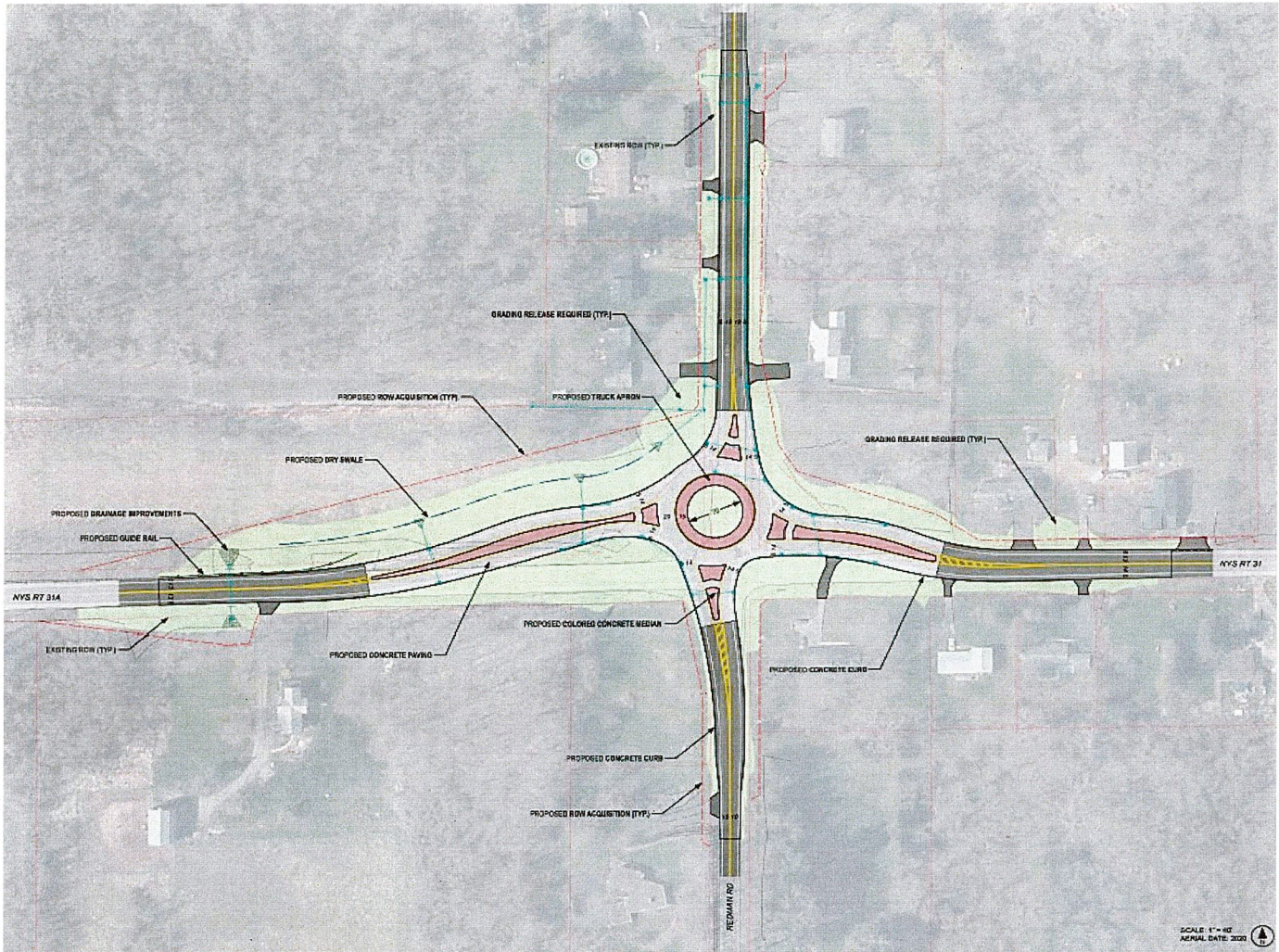
Phase 2A 2028 Roundabout Construction
